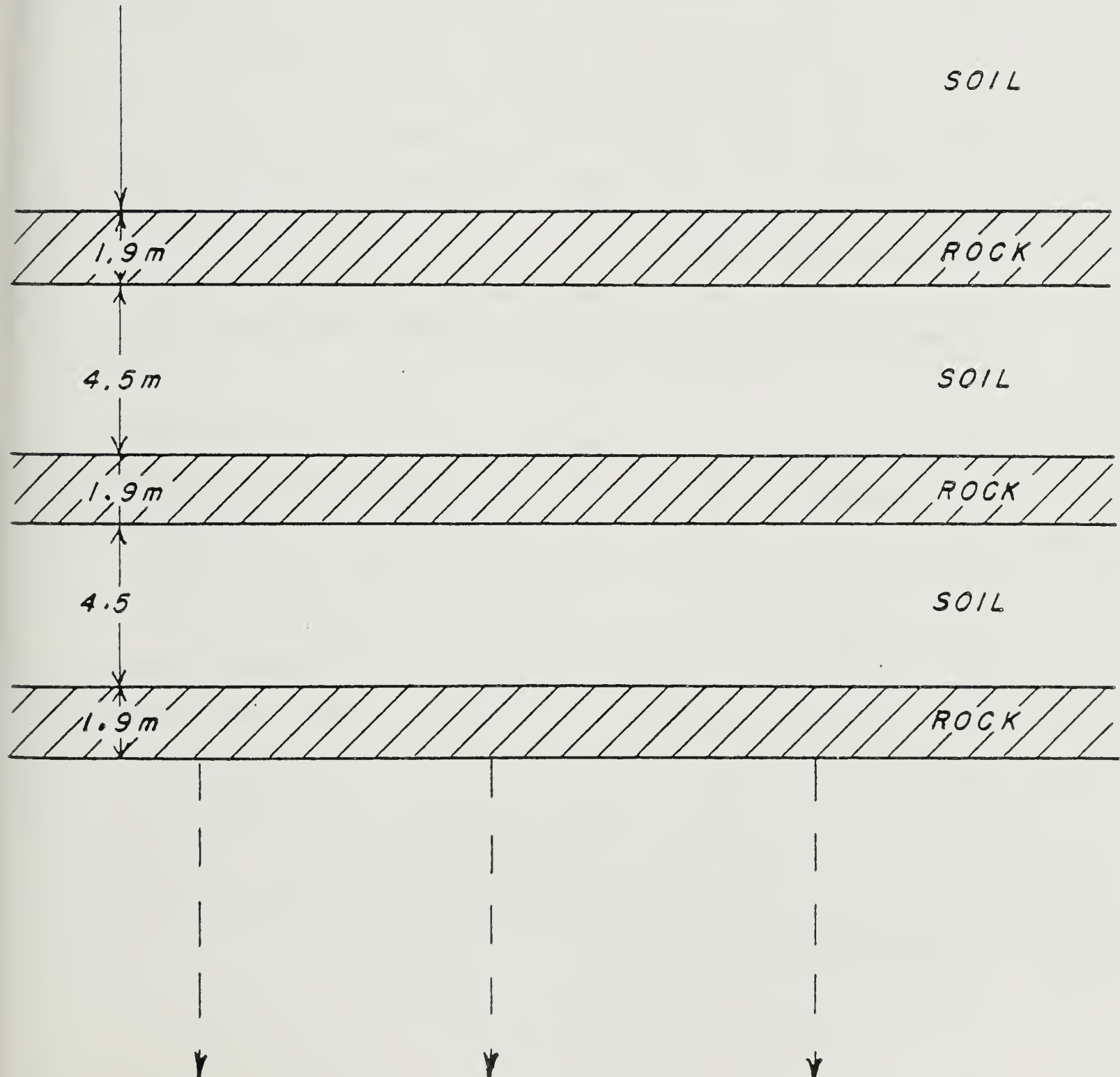
A schematic drawing of the multilayered models of the upper lunar crust. The designated physical properties are based on lunar in situ experiments and measurements on returned lunar samples.
